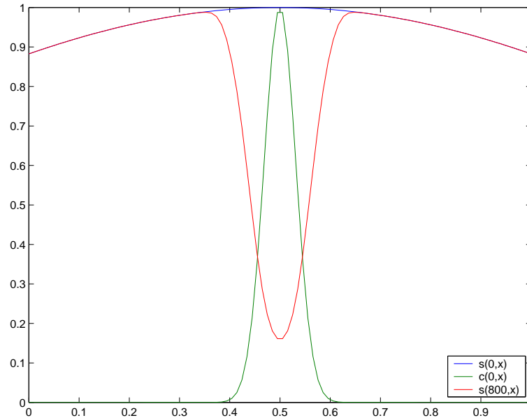
Figure 2: This figure corresponds to the local case with \alpha = 0.0005 . The green curve corresponds to the initial distribution of bacteria, the blue curve corresponds to the initial distribution of susceptible hens, and red curve corresponds to distribution of S -infectious at time t=800 .
