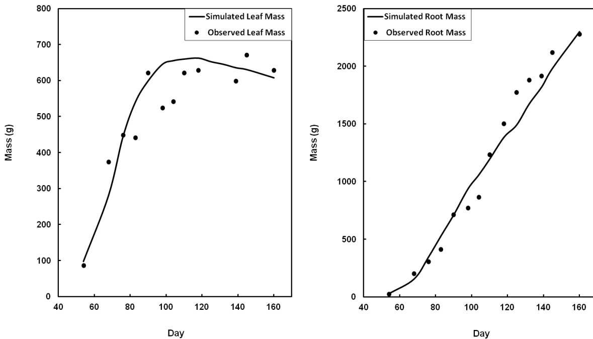
FIGURE 3. Comparison of simulated leaf mass (on the left) and root mass (on the right) with experimental data
