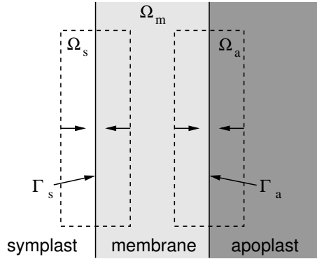
FIGURE 3. Scheme of the method used to obtain the transmission conditions. Small domains \Omega_s and \Omega_a enclosing the interface symplast-membrane and membrane-apoplast, respectively, are reduced to the surfaces \Gamma_s and \Gamma_a . The membrane is represented by the domain \Omega_m .
