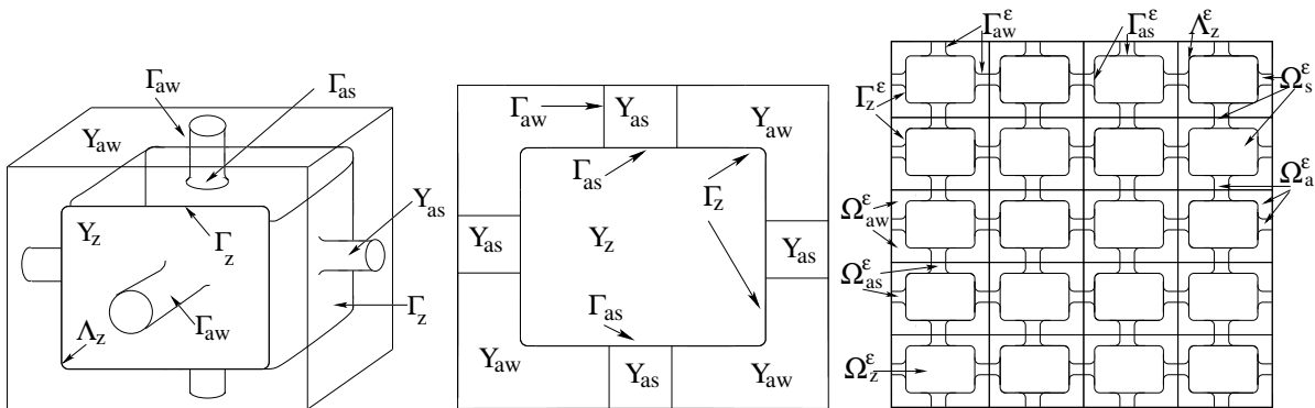
FIGURE 5. Left: unit cell Y . Center: 2D cross-section of a unit cell Y . Right: 2D cross-section of a plant tissue \Omega .
