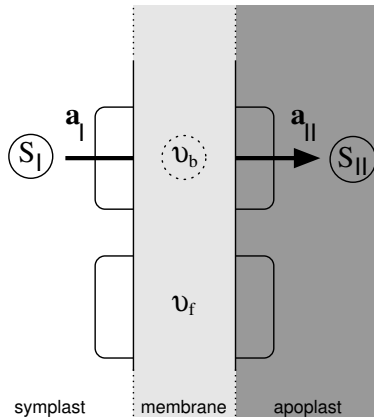
FIGURE 4. Depiction of the mechanism assumed for protein mediated transport, where a transport direction from symplast to apoplast is shown exemplarily.
