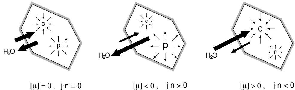
FIGURE 1. Scheme of water flux into and out of a single cell. The flux is proportional to the jump in chemical potential [\mu] , which depends on internal pressure p and solute concentration c .
