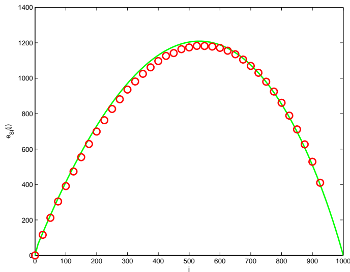
FIGURE 7. The (j, e_{SI}(j)) curve obtained from simulation (o) and from recursion (4.5) (continuous curve) in the case of a regular random graph with N = 1000 , \tau = 2 , \gamma = 1 , n = 6 .
