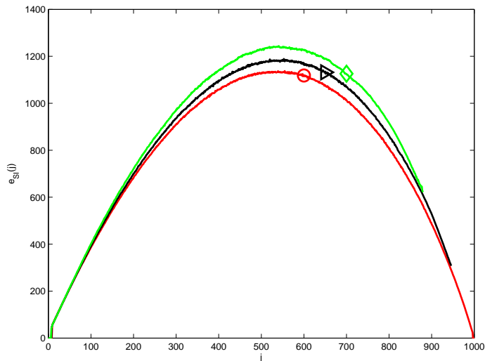
FIGURE 5. The (j, e_{SI}(j)) curves in the case of a regular random graph for different values of \tau from simulation ( \tau = 1 ( \diamond ), \tau = 2 ( \blacktriangleright ), \tau = 10 ( \circ )).
