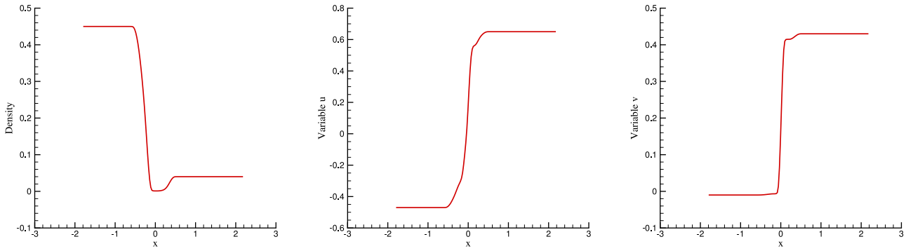
FIGURE 7. Numerical results of \rho , u and v for data 2 at \epsilon = 0.003 .
