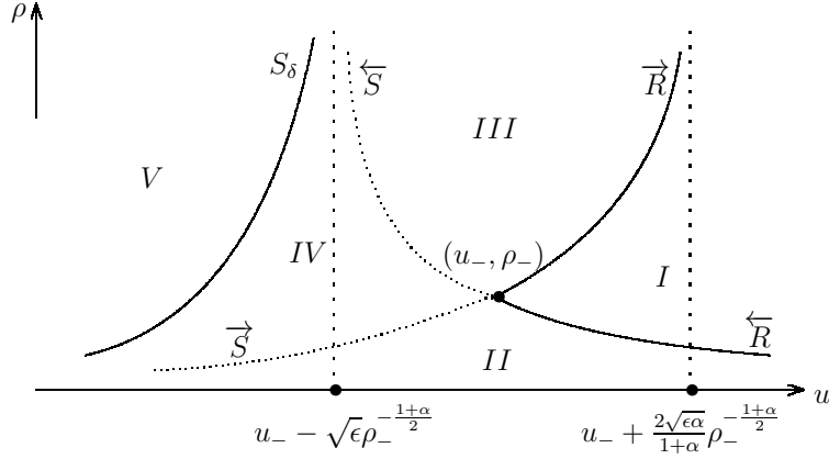
FIGURE 1. The projections of wave curves for (1.1) and (1.3) onto (u, \rho) plane.
