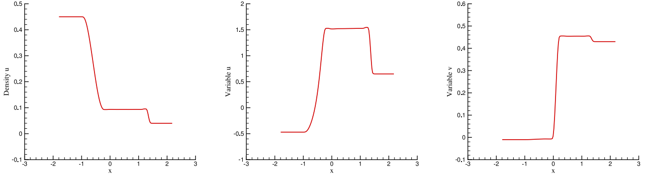
FIGURE 6. Numerical results of \rho , u and v for data 2 at \epsilon = 1 .
