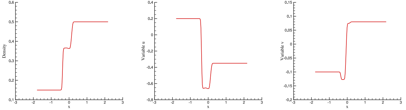
FIGURE 3. Numerical results of \rho , u and v for data 1 at \epsilon = 1 .
