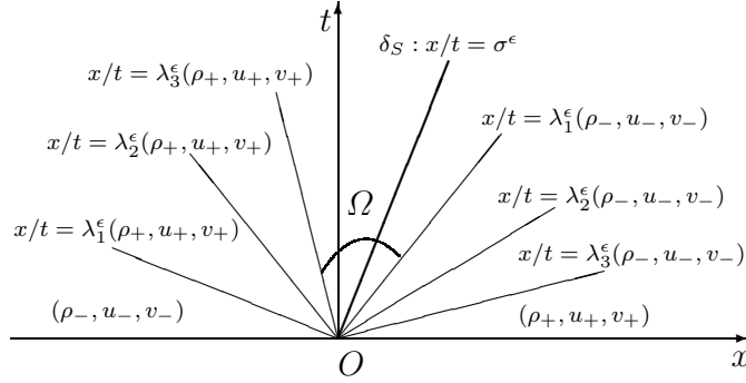
FIGURE 2. Analysis of characteristics for delta-shock of (1.1) and (1.3).
