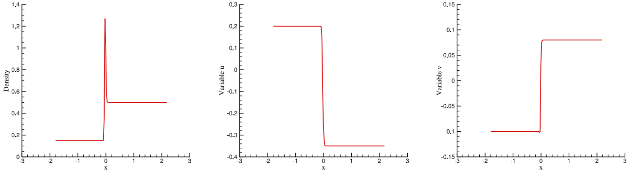
FIGURE 4. Numerical results of \rho , u and v for data 1 at \epsilon = 0.0089 .
