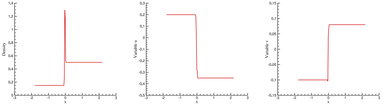
FIGURE 5. Numerical results of \rho , u and v for data 1 at \epsilon = 0.001 .
