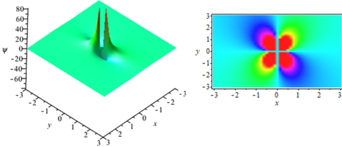
Fig. 5. Rational solution when a_4 = 0 , a_5 = -2 , a_6 = 1 , a_8 = 0 , and t = 0 .
