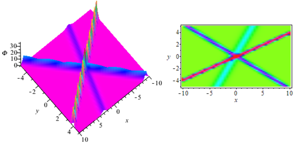
Fig. 3. Triple soliton solution when \kappa_1 = 3 , \tau_1 = -2 , \kappa_2 = -5 , \tau_2 = -9 , \kappa_3 = -8 , \tau_3 = 20 , and t = 0 .
