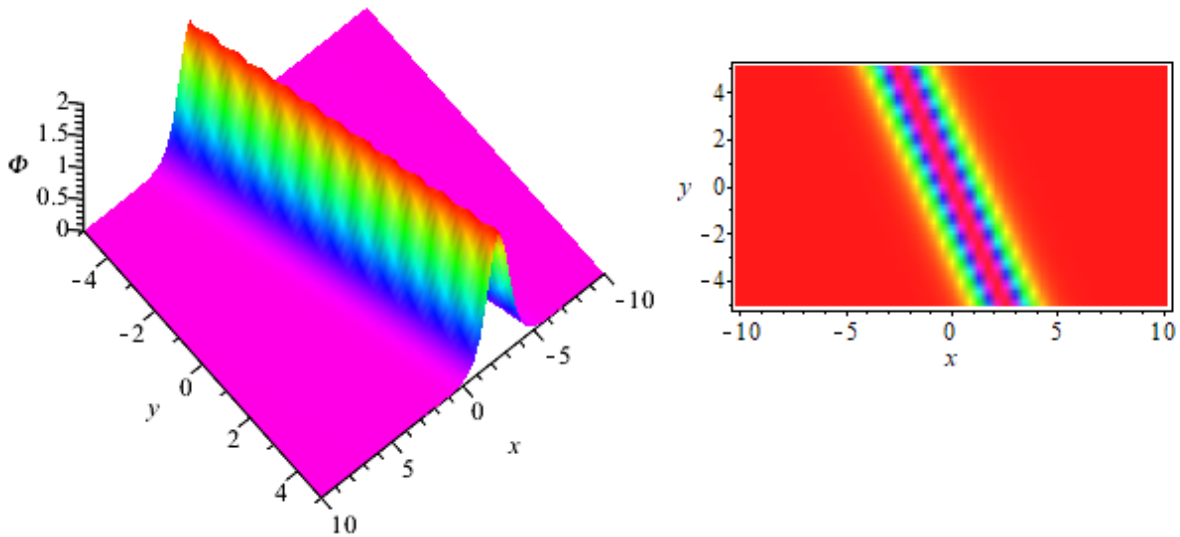
Fig. 1. Single soliton solution when \kappa_1 = 1 , \tau_1 = 2 , and t = 0 .
