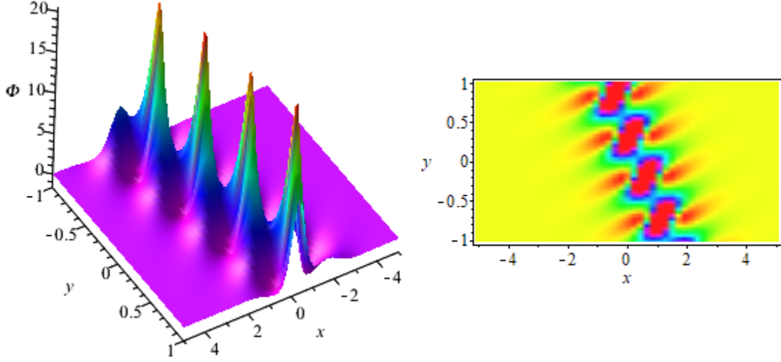
Fig. 6. Complexiton solution when k_1 = -2 , k_2 = -2 , r_1 = -2 , r_2 = 10 , and t = 0 .
