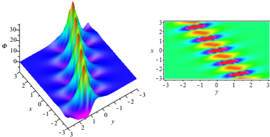
Fig. 4. Breather solution when a_1 = 1 , a_2 = 2 , a_4 = 0 , a_5 = -2 , a_6 = 1 , a_8 = 0 , k = 1 , h = -2 , b_0 = -1 , and t = 0 .
