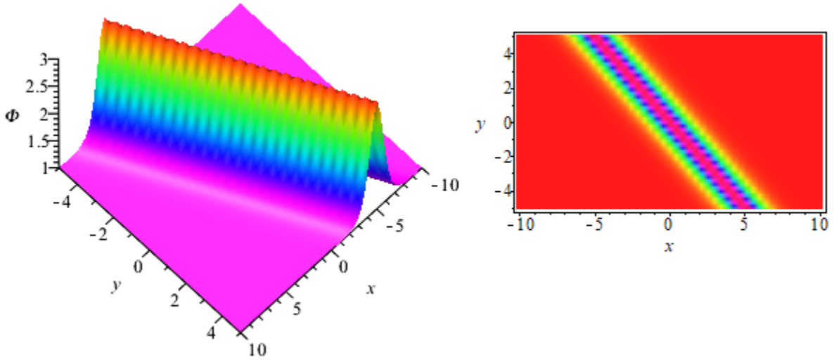
Fig. 7. Hyperbolic solution (68) when A_0 = 1 , \kappa = 1 , \tau = 1 , and t = 0 .
