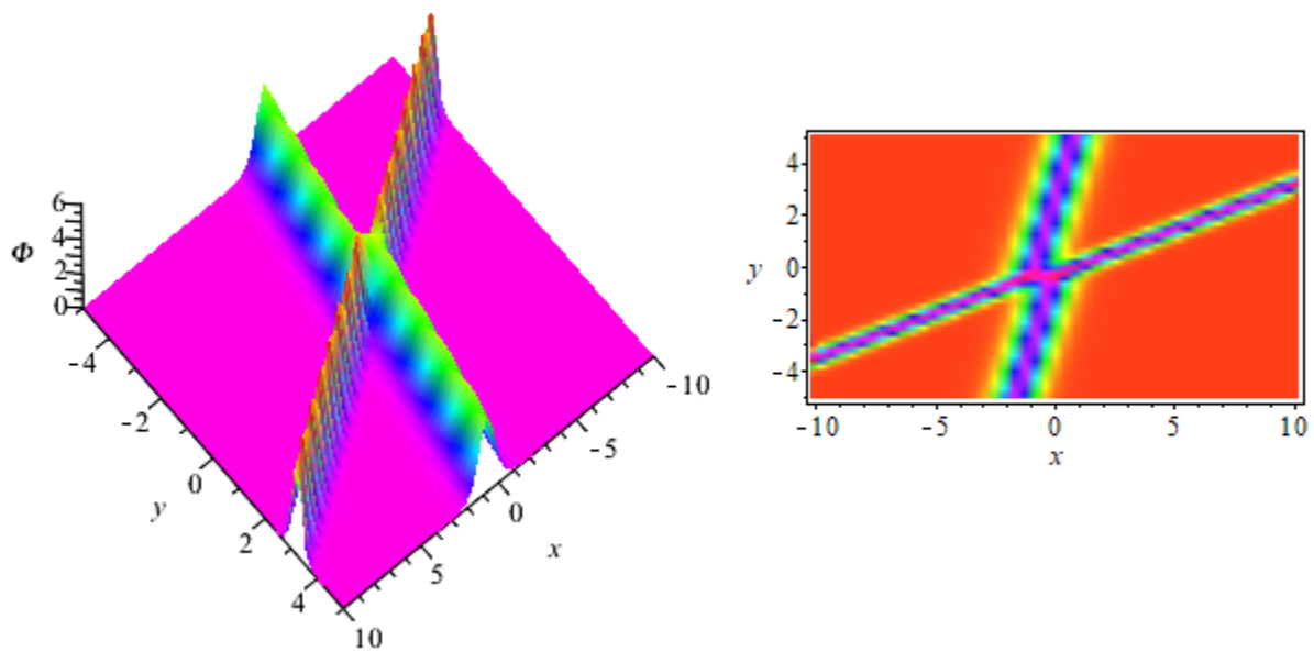
Fig. 2. Double soliton solution when \kappa_1 = -3.5 , \tau_1 = 10 , \kappa_2 = 3 , \tau_2 = -1 , and t = 0 .
